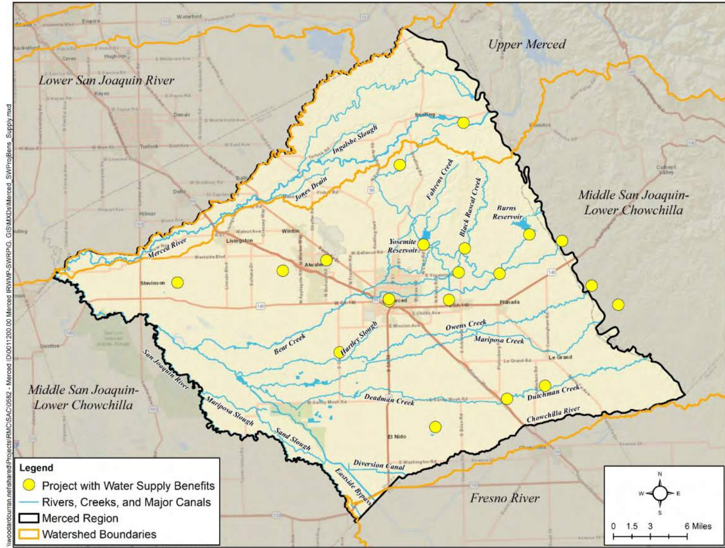
Figure 5-2: SWRP Projects Providing Water Supply Benefits via Stormwater Capture and Use
