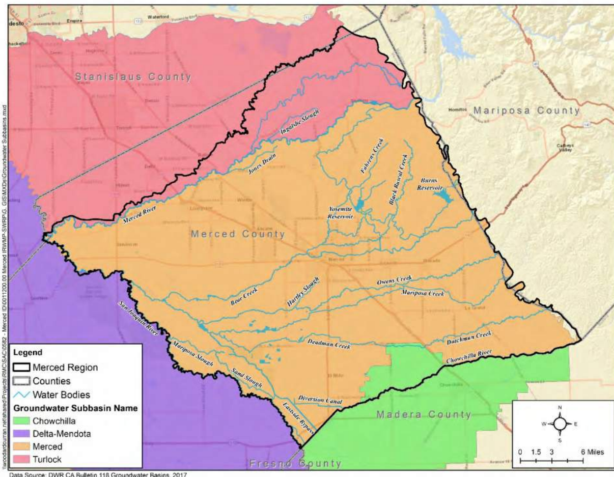
Figure 2-10: Groundwater Subbasins in the Merced Region
