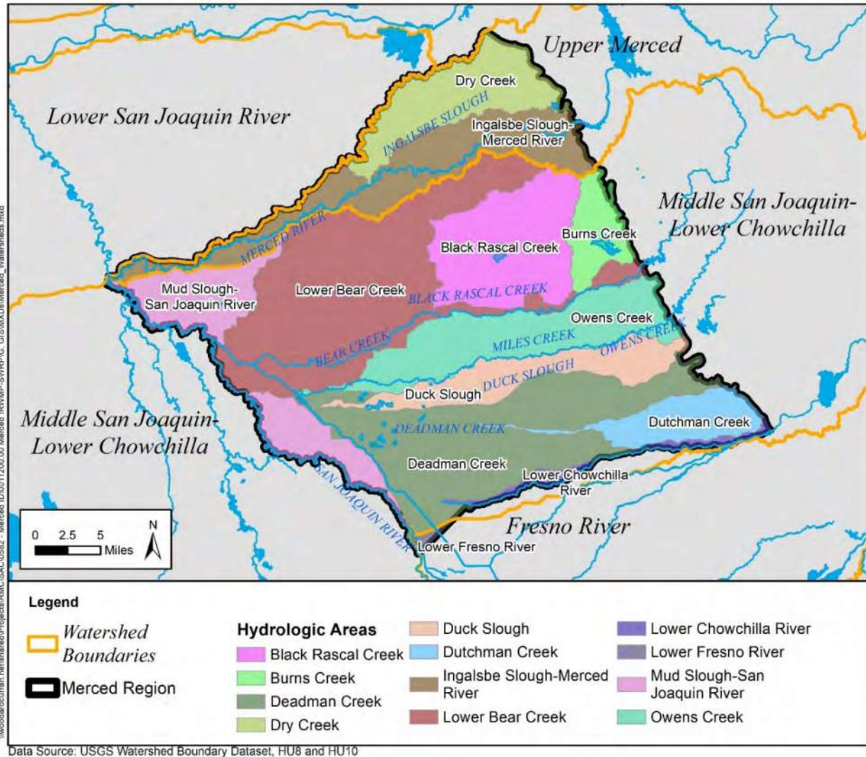
Figure 2-2: Watersheds within the Merced Region
